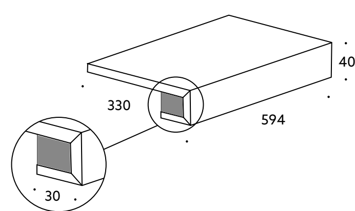
Costa retta 60 ≠6 mm | ≠12 mm
